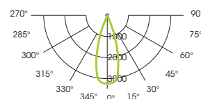
2x40° (1/10)
